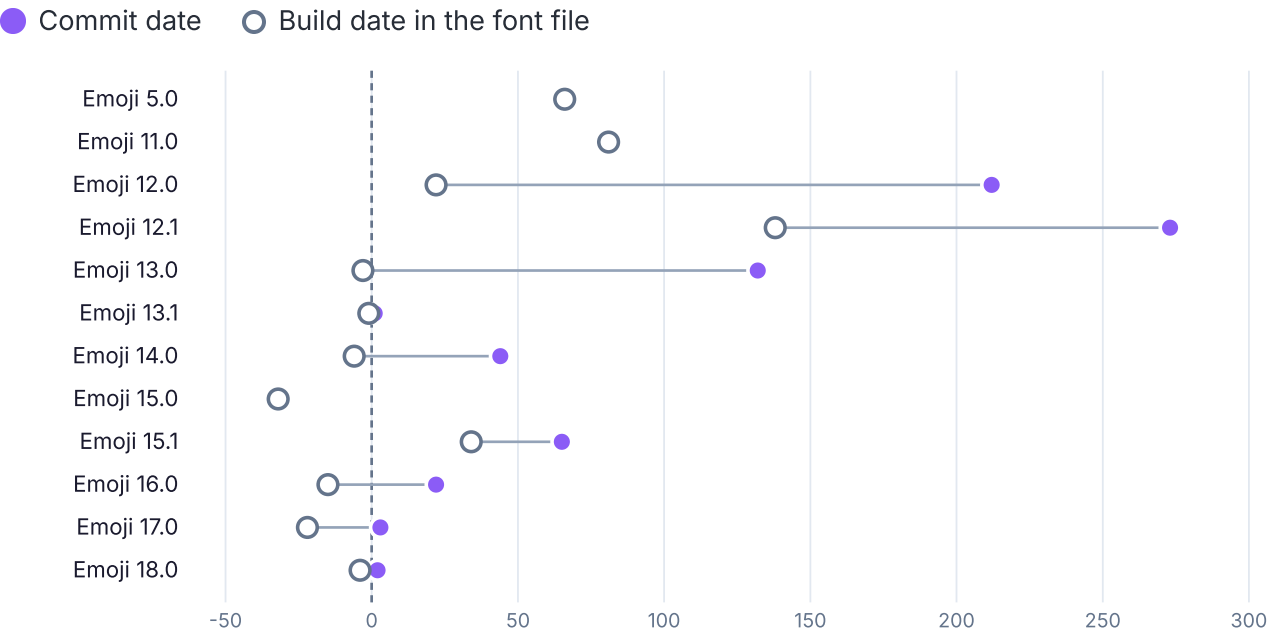
Figure 2. Days from an Emoji release to the first Noto Color Emoji binary that composes its sequences. Filled dot: date the binary was committed to the font’s repository. Ring: date stamped inside the font file. Negative means the font came first.
