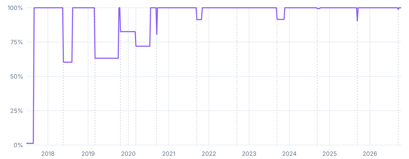
Figure 3. Share of already-standardized emoji (Emoji 5.0 onward) that the newest committed Noto Color Emoji binary can compose, every day from 2017-06-20 to 2026-10-12. Each vertical line is an Emoji release.
