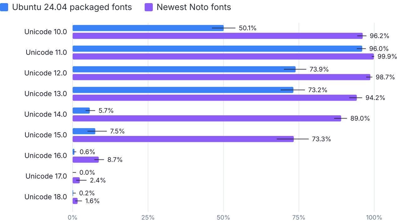
Figure 1. Share of code points drawn as intended, by Unicode release. Chromium 155 on Linux, with the fonts Ubuntu 24.04 packages and with the newest Noto fonts. Whiskers are 95% intervals.
